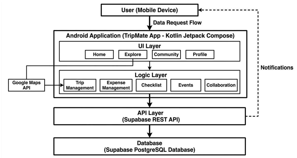
Fig 3.1.1 Architecture Diagram
